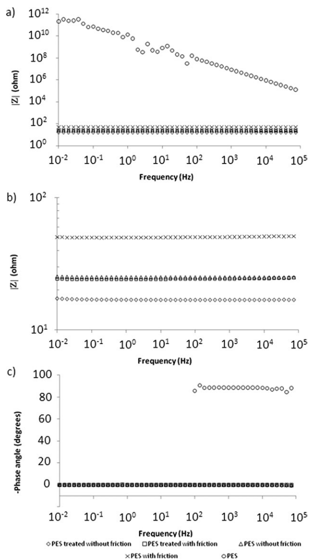
Figure 8. Bode plots for PES, untreated/treated PES + PPy/PW 12 O 40 3- before and after rubbing fastness tests. Sample located between two copper electrodes. Frequency range from 105 Hz to 10 -2 Hz.
