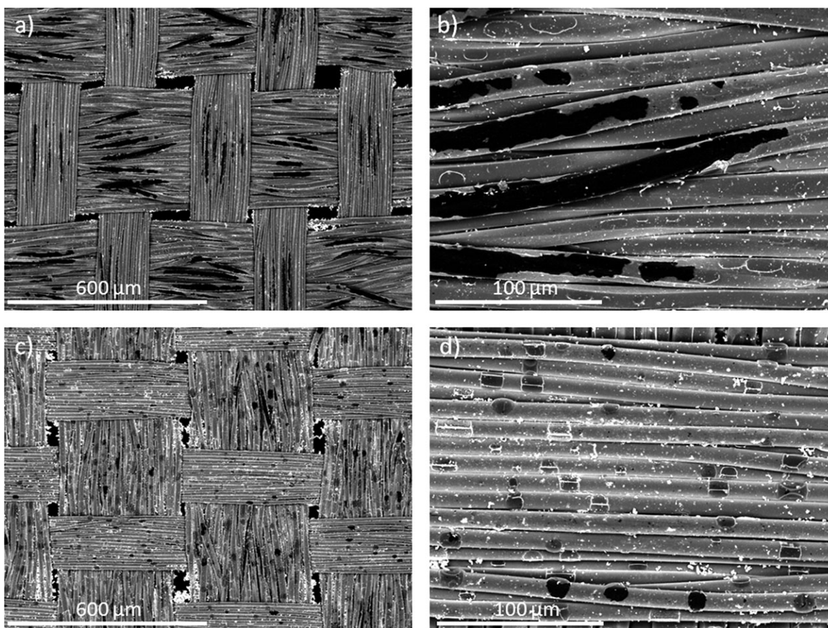
Figure 6. SEM micrographs obtained with backscattered electrons (BSE) of: PES without treatment + PPy/PW 12 O 40 3- after rubbing test; (a) ( \times 100 ), (b) ( \times 500 ). PES with plasma treatment ( 4500 \text{ W min}^{-1} \text{ m}^{-2} ) + PPy/PW 12 O 40 3- after rubbing fastness test; (c) ( \times 100 ), (d) ( \times 500 ).
