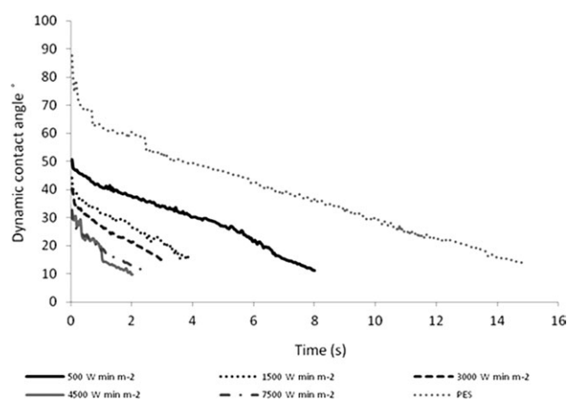
Figure 1. Dynamic contact angle ( ^\circ ) measurements for polyester fabrics treated with different plasma dosages.
