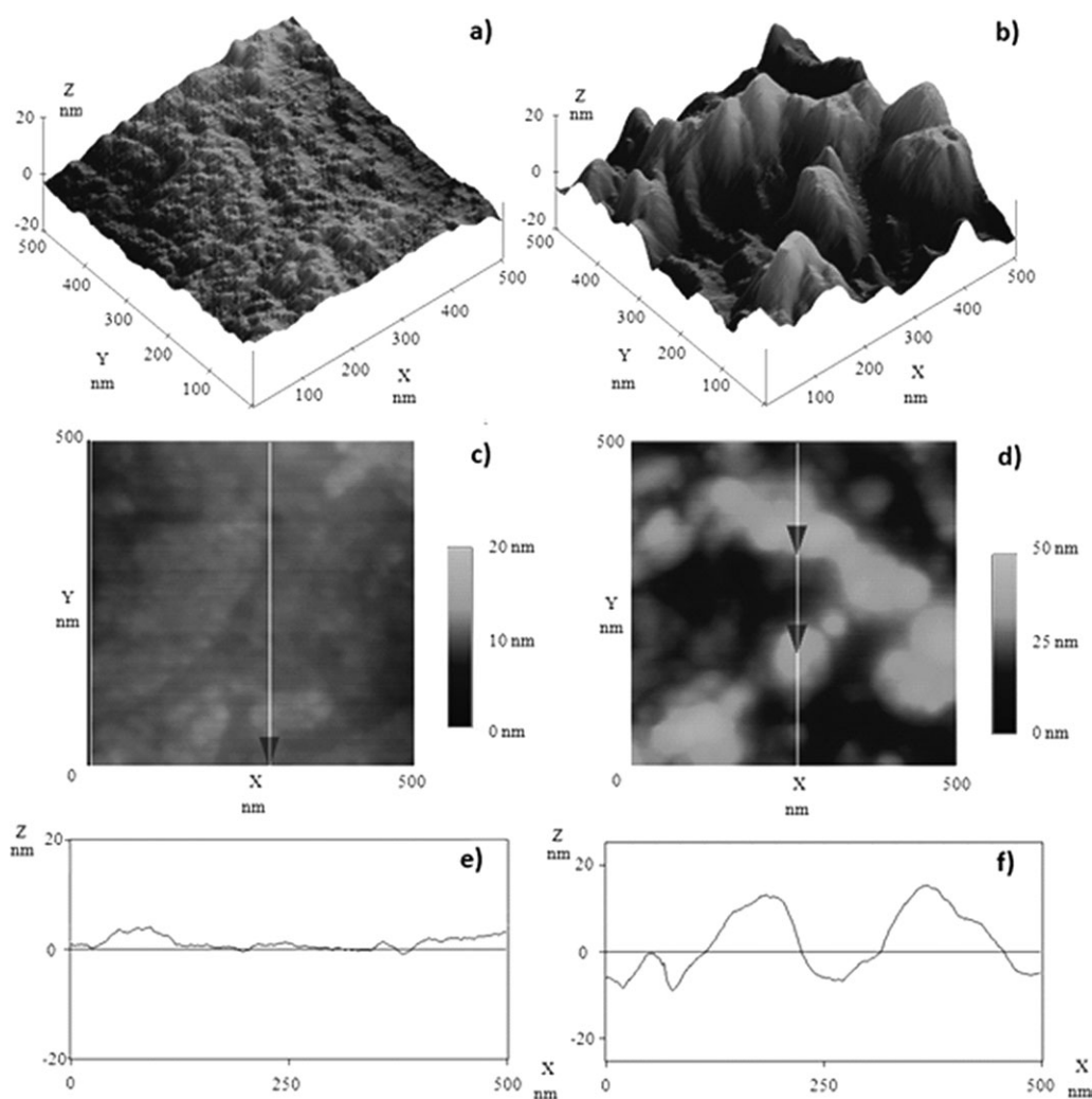
Figure 4. AFM 3D topographic representations of untreated (a) and plasma treated polyester ( 4500 \text{ W min}^{-1} \text{ m}^{-2} ) (b). AFM 2D roughness profiles of untreated (c) and treated polyester (d). Section roughness profile of untreated (e) and treated polyester (f).
