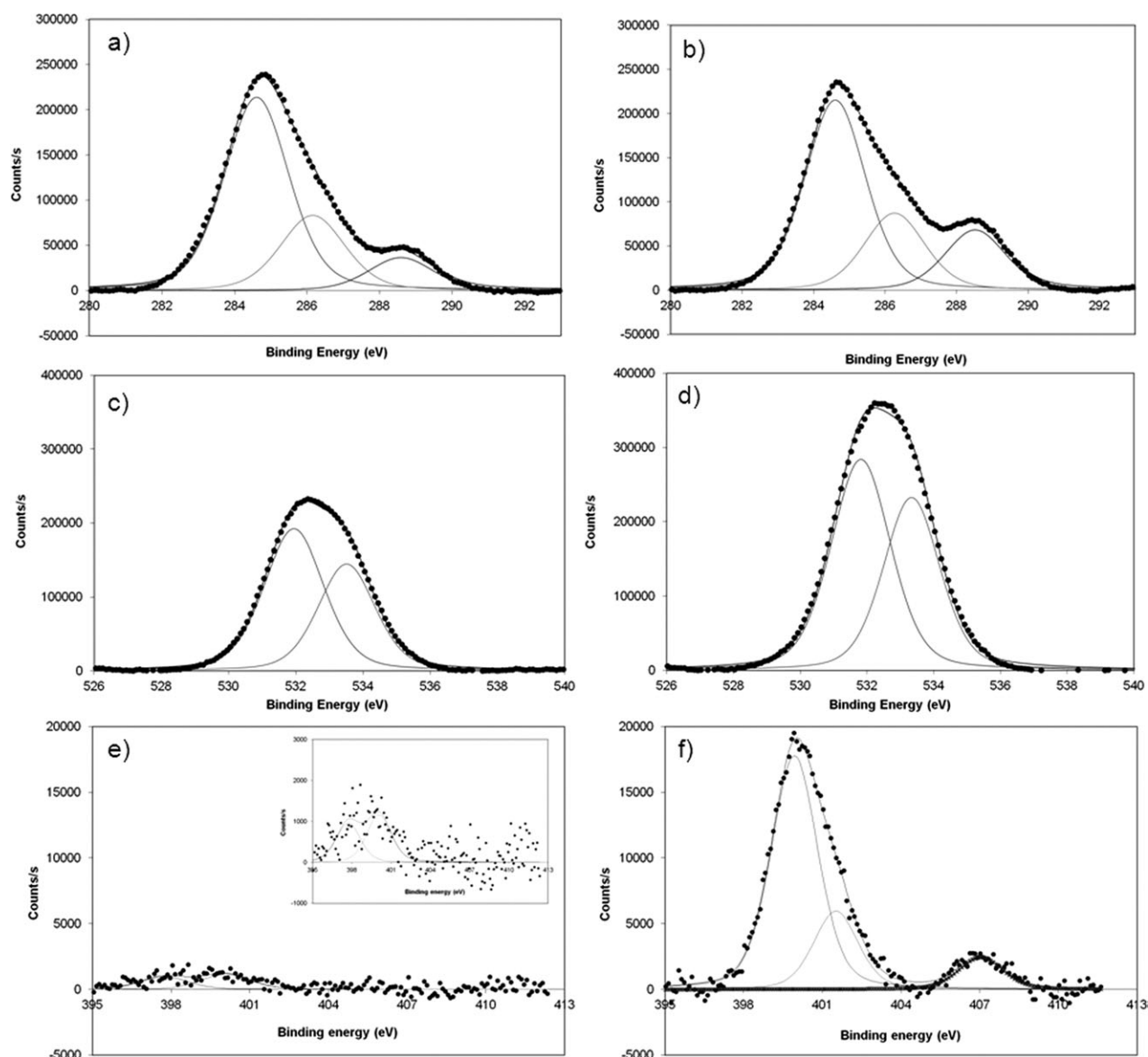
Figure 2. C1s (a,b), O1s (c, d), and N1s (e, f) XPS high resolution spectra for untreated (a, c, e) and plasma treated polyester (b, d, f).
