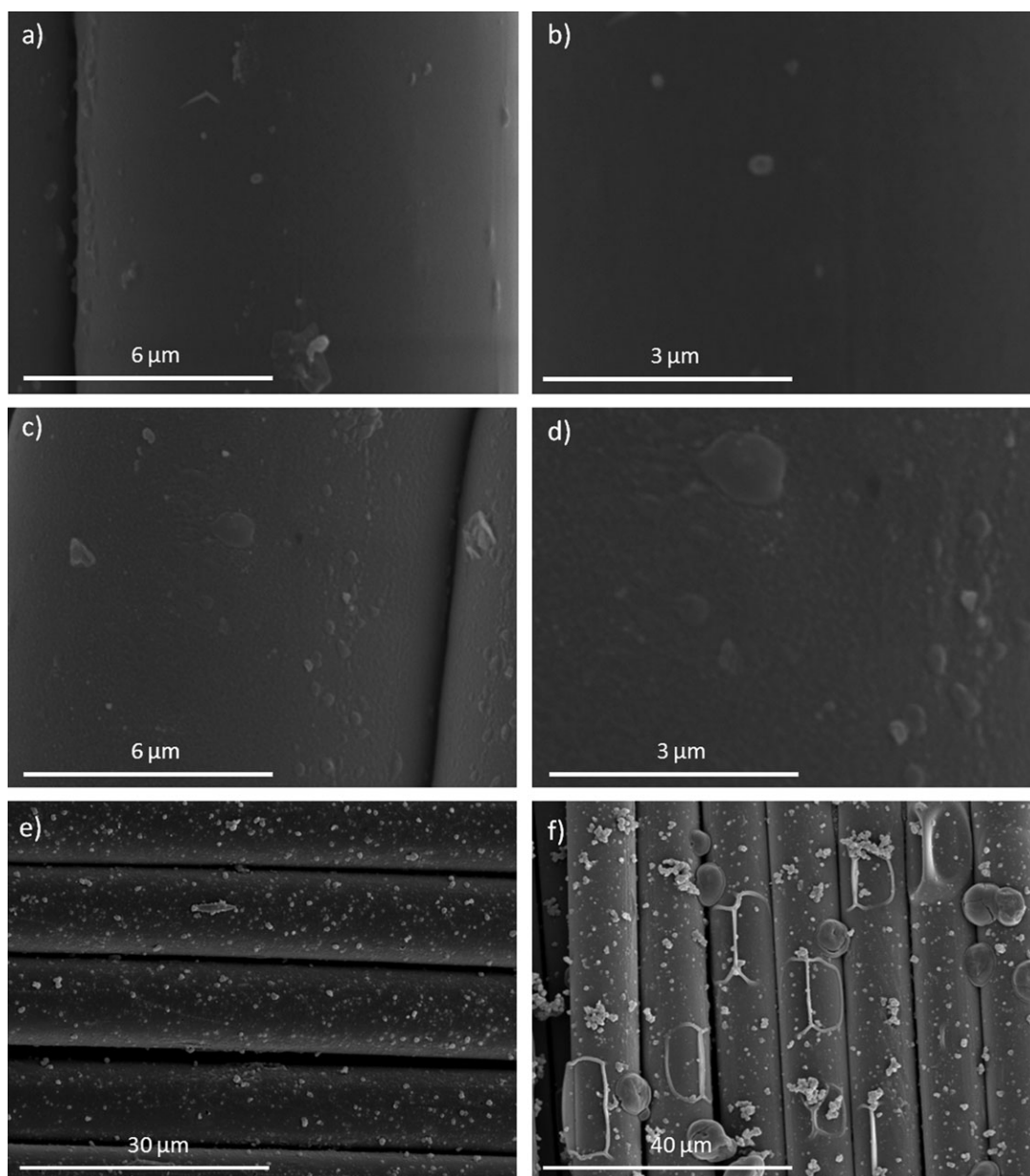
Figure 3. SEM micrographs of: (a) PES without treatment ( \times 10,000 ), (b) PES without treatment ( \times 20,000 ), (c) PES treated 4500 \text{ W min}^{-1} \text{ m}^{-2} ( \times 10,000 ), (d) PES treated 4500 \text{ W min}^{-1} \text{ m}^{-2} ( \times 20,000 ), (e) PES without treatment + PPy/PW 12 O 40 3- ( \times 2000 ), (f) PES treated 4500 \text{ W min}^{-1} \text{ m}^{-2} + PPy/PW 12 O 40 3- ( \times 1500 ).
