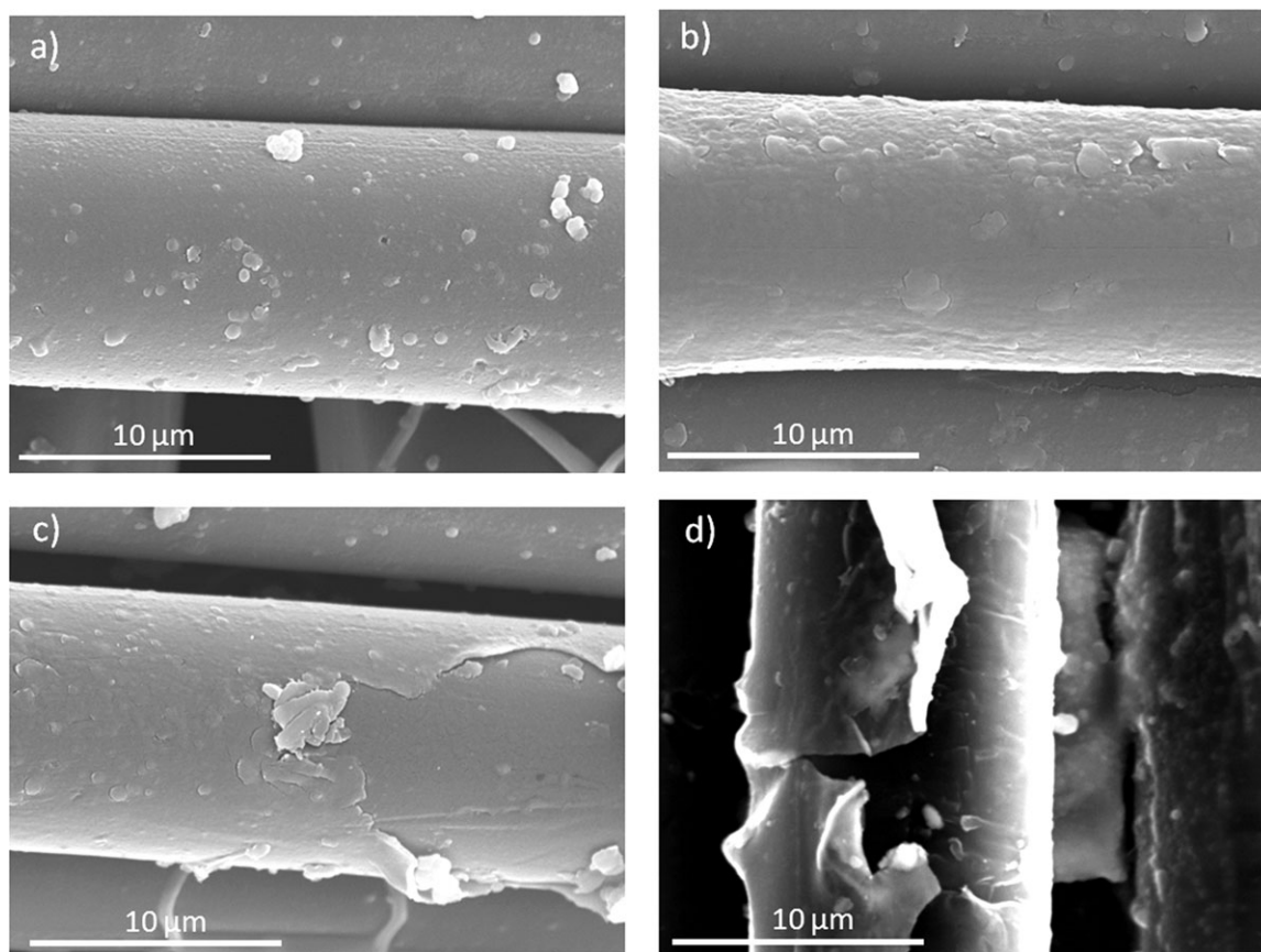
Figure 7. SEM micrographs obtained with secondary electrons (SE) of: PES with plasma treatment ( 4500 \text{ W min}^{-1} \text{ m}^{-2} ) + PPy/PW 12 O 40 3- after rubbing fastness test; (a) ( \times 5000 ), (b) ( \times 5000 ), (c) ( \times 5000 ). PES without treatment + PPy/PW 12 O 40 3- after rubbing fastness test; (d) ( \times 5000 ).
